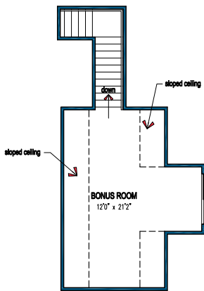
Second Floor 378 Sq. Ft.
